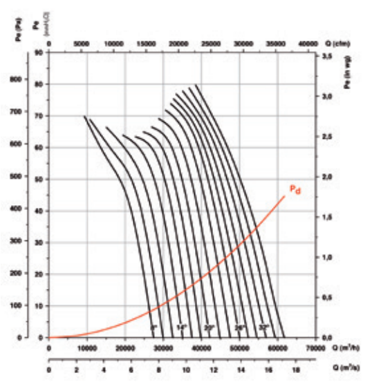
HTP-90-4T
