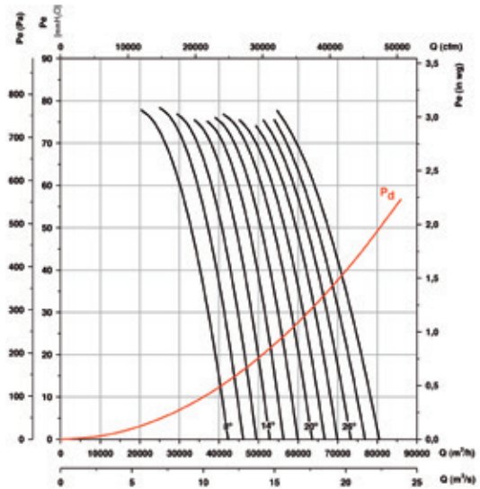
HTP-100-4T
