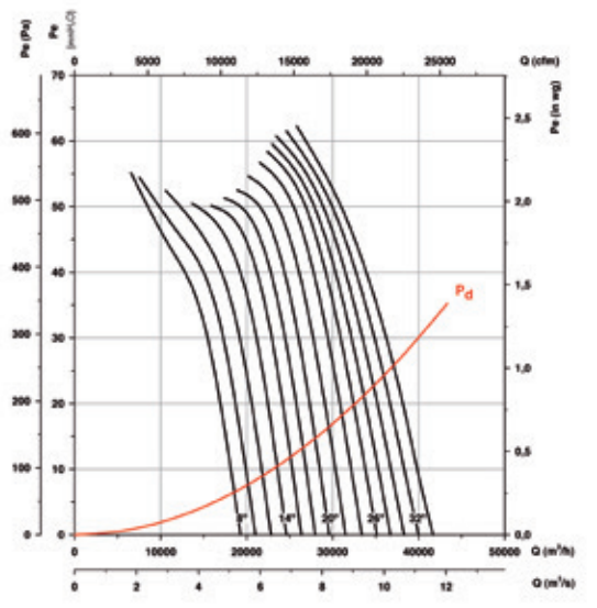
HTP-80-4T
